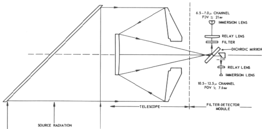
Figure 1: Nimbus IV THIR Optical Schematic
