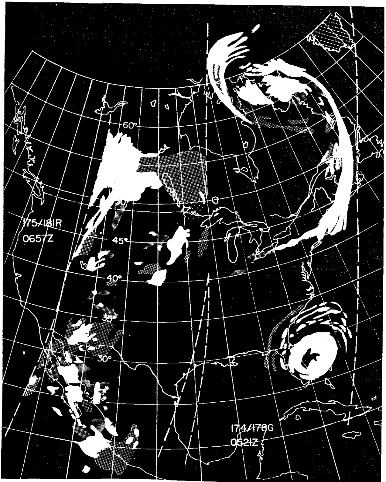
Figure 9-63—Rectified HRIR Data for 9 September 1964 (See Reference 44 for Shading Convention for Rectified HRIR Data)
