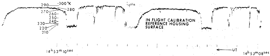
Figure 3-4--Portion of an analog record showing nearly two HRIR scan cycles.
