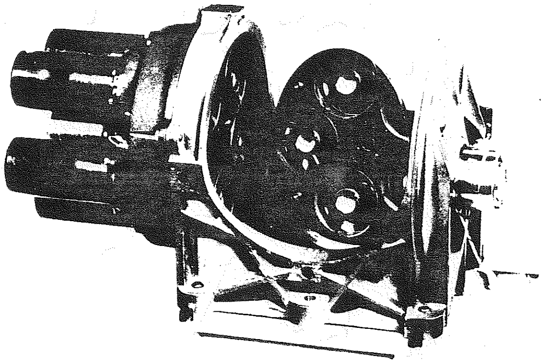
Figure 4-1—MRIR Radiometer
