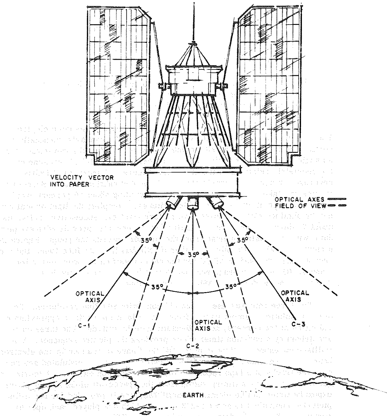
Figure 2-1—Schematic of AVCS Optics
