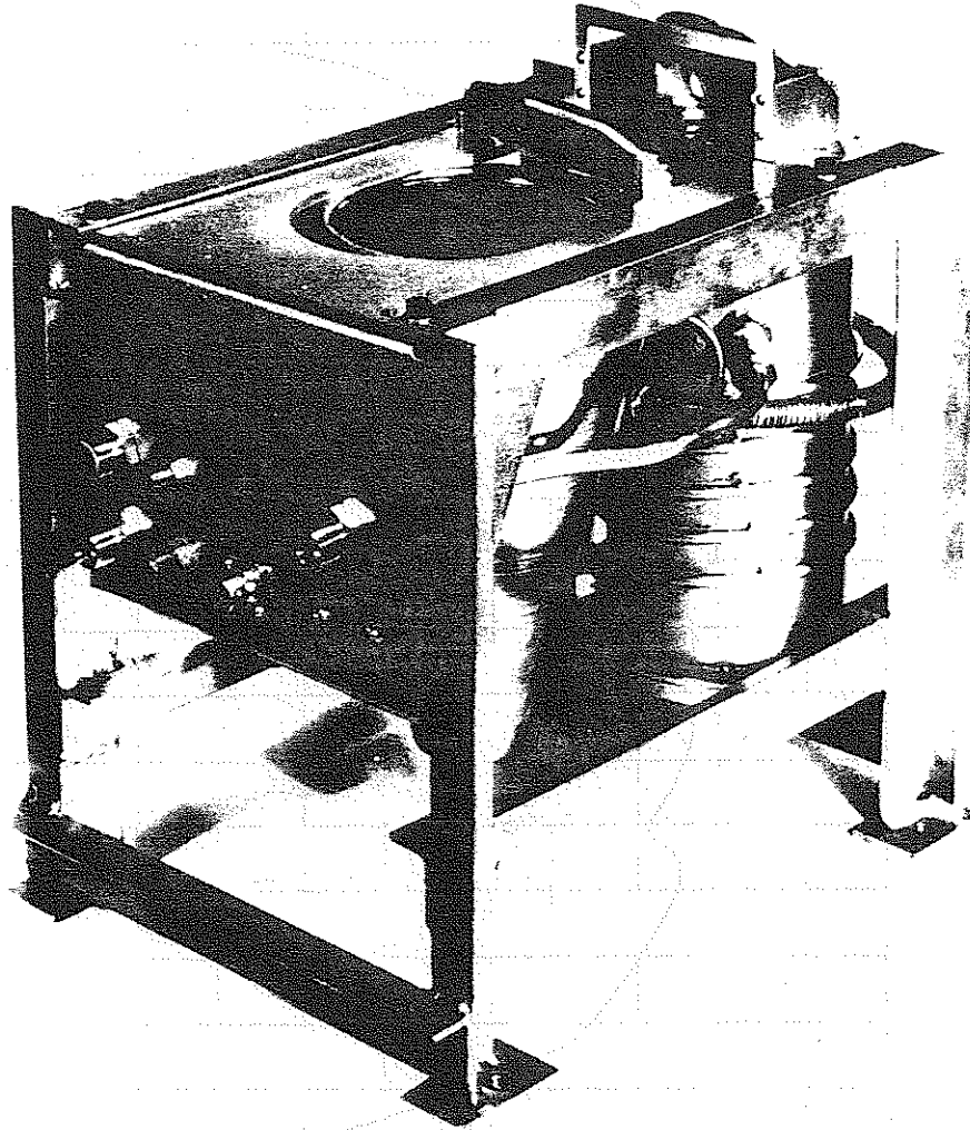
Figure 4-14-MRIR Calibration Target Assembly
