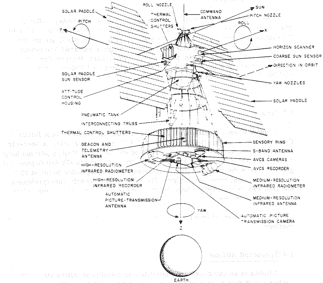
Figure 1-1-Nimbus II Spacecraft
