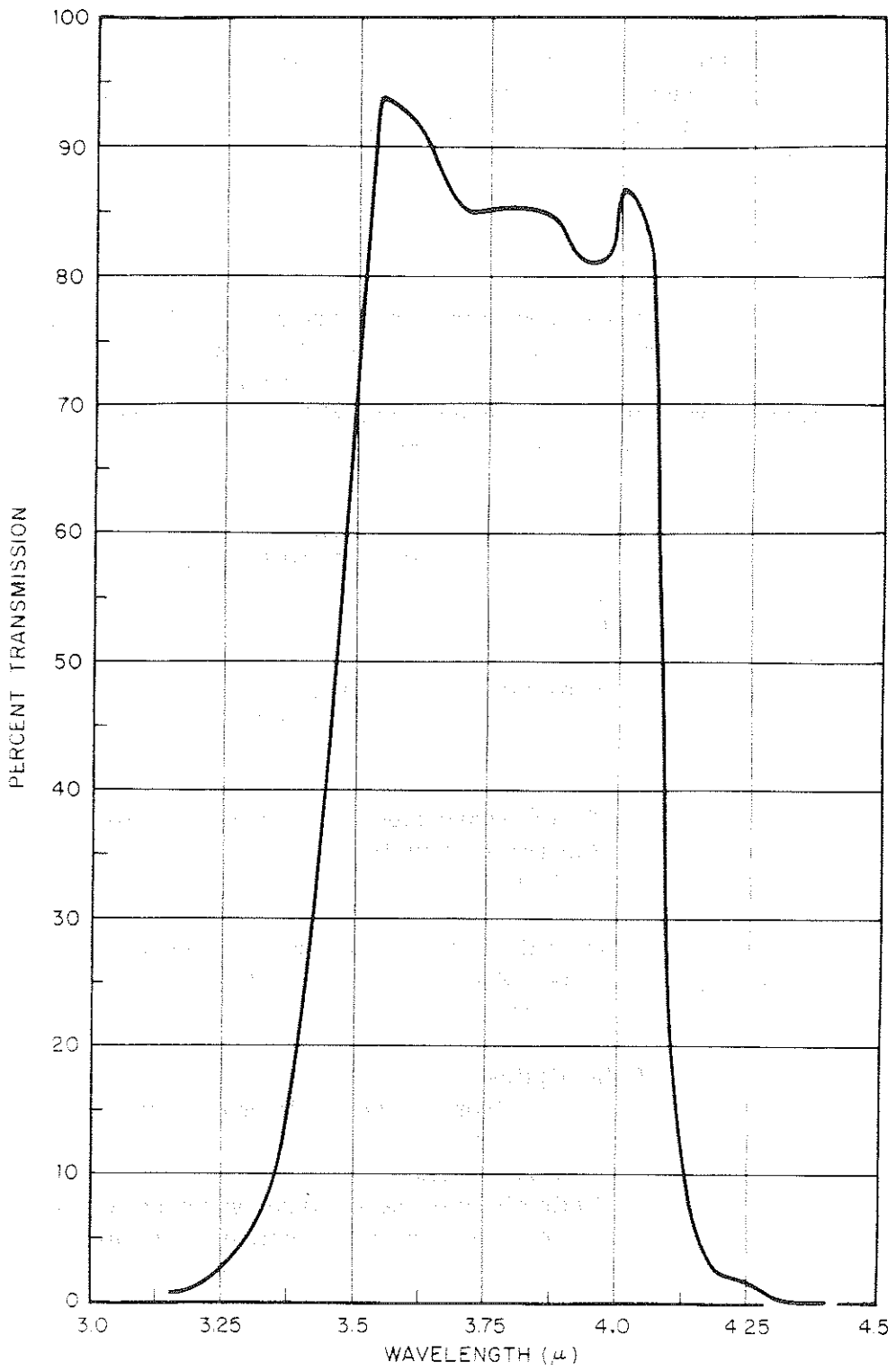
Figure 3-12—The effective spectral response of the HRIR versus wavelength
