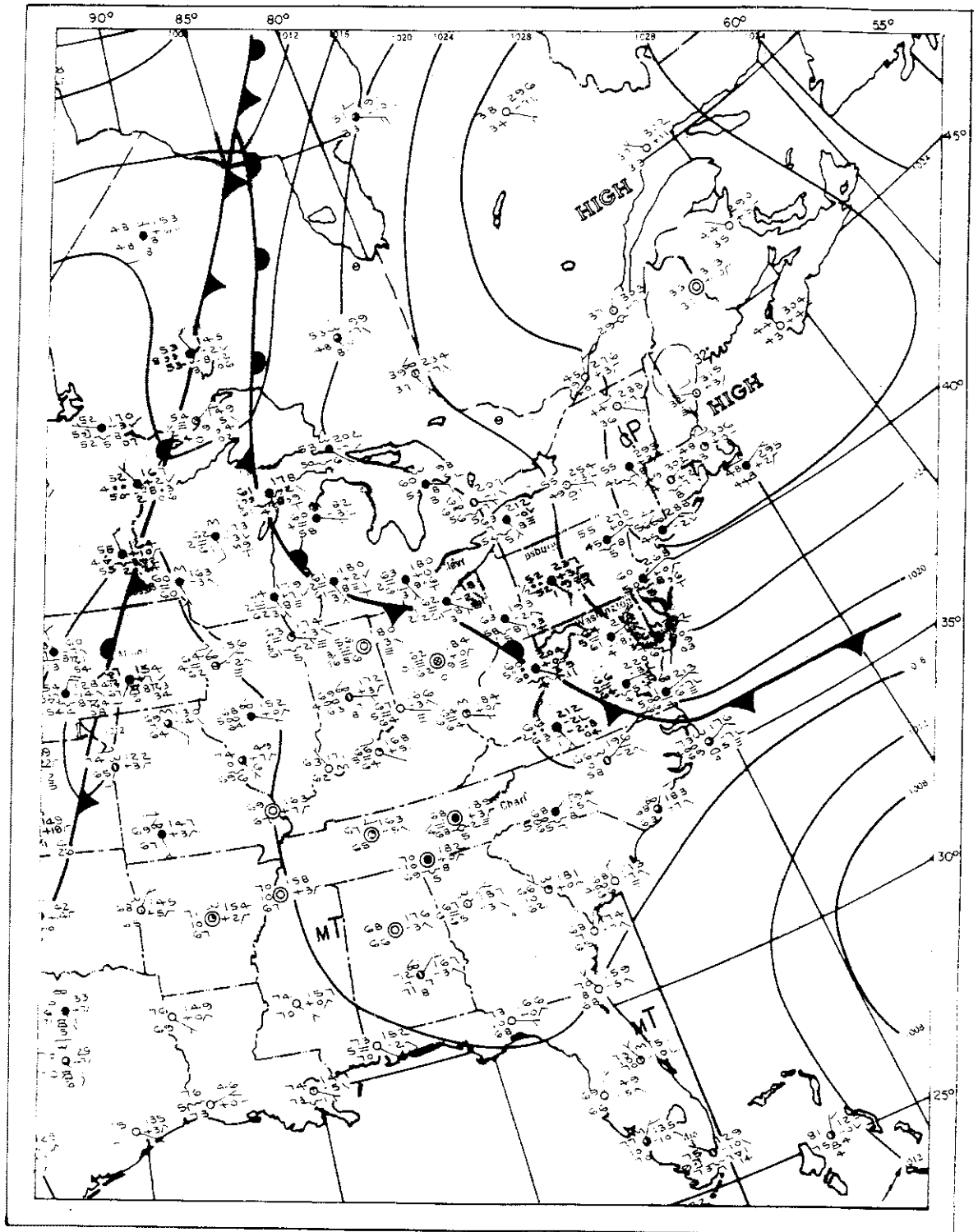
Figure 9-80—Surface Weather Map at 0600 UT, 20 September 1964
