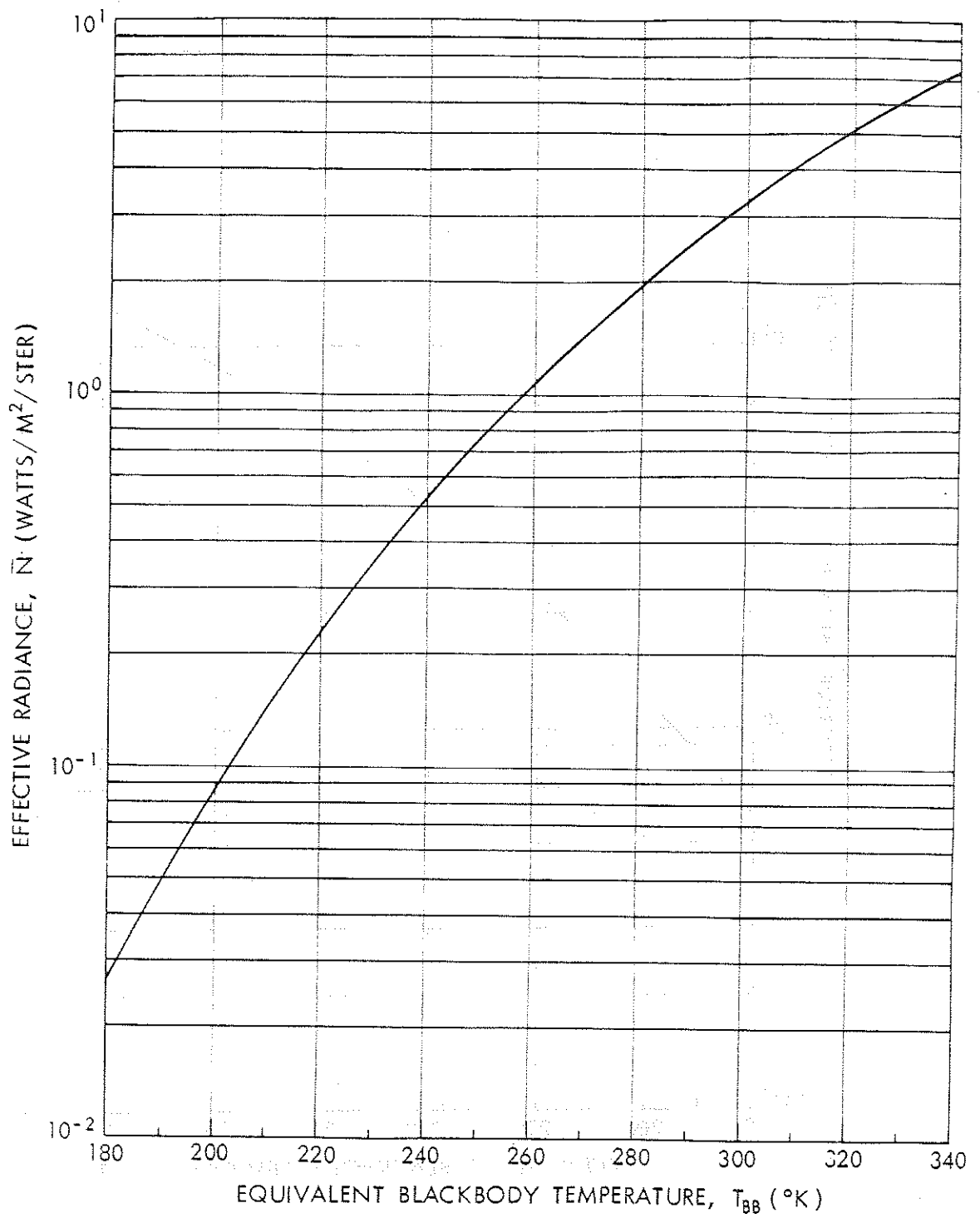
Figure 4-5-N vs. T_{BB} for 6.4-6.9 Micron Channel
