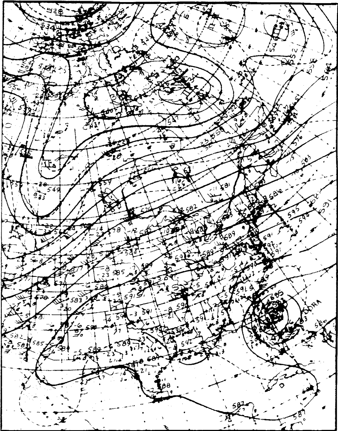
Figure 9-64-NMC 500 mb Analysis, 1200 UT, 9 September 1964
