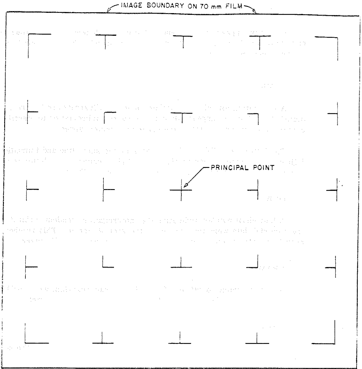
Figure 2-5—Nimbus AVCS Fiducial Matrix (This display is enlarged approximately three times the actual image size)
