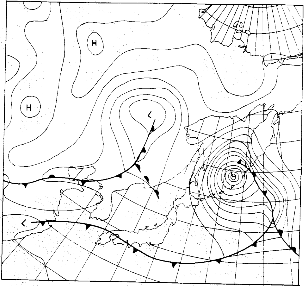
Figure 9-69-NMC Surface Analysis, 1200 UT, 14 September 1964
