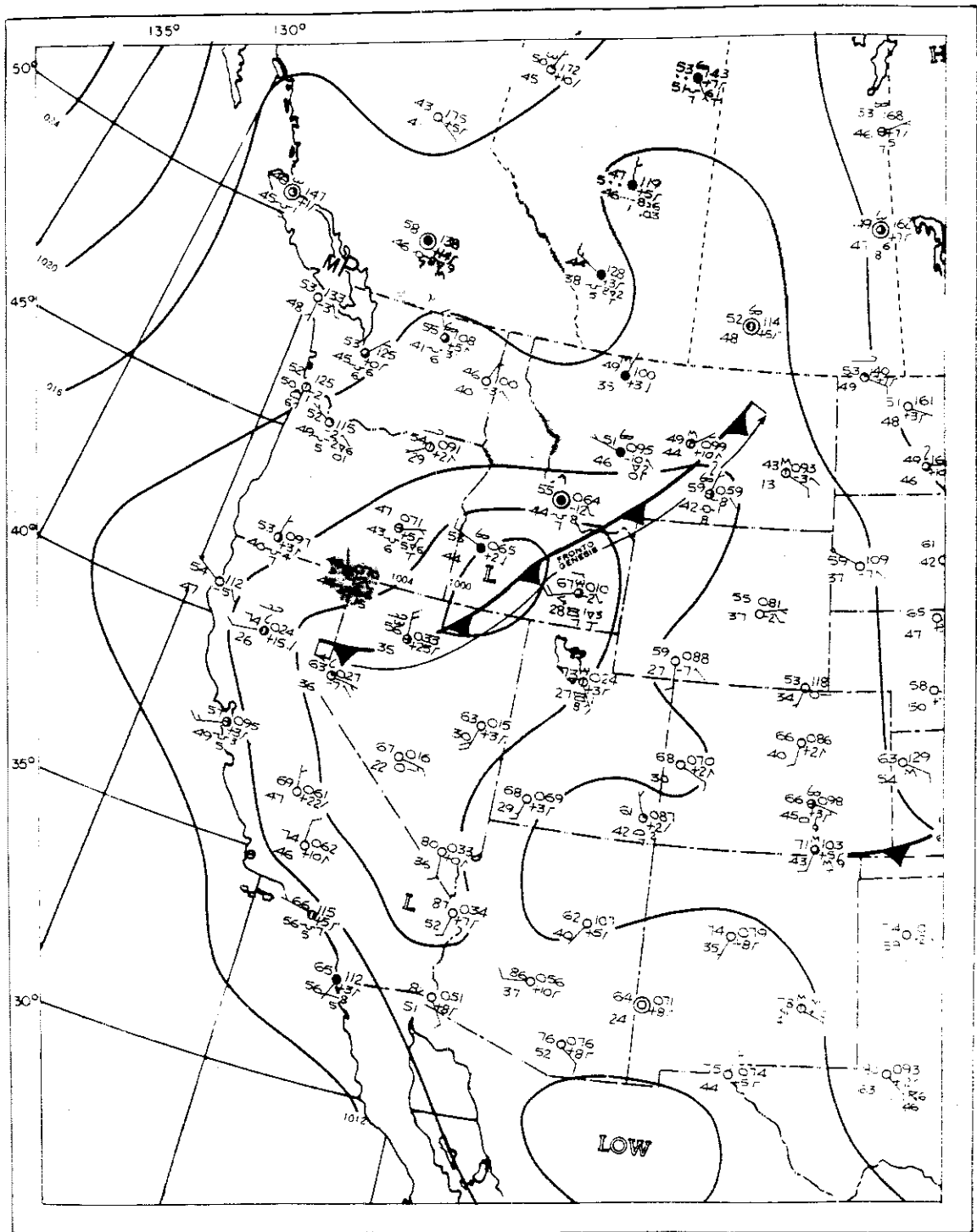
Figure 9-77—Surface Weather Map for 0600 UT, 31 August 1964
