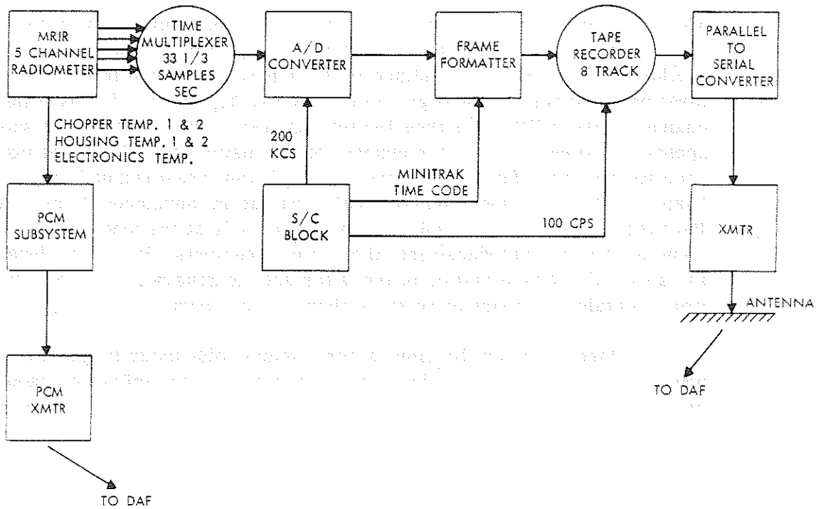
Figure 4-4—Block Diagram of S/C Portion of MRIR System
