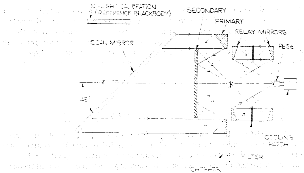
Figure 3-3—Schematic of the HRIR optical system.
