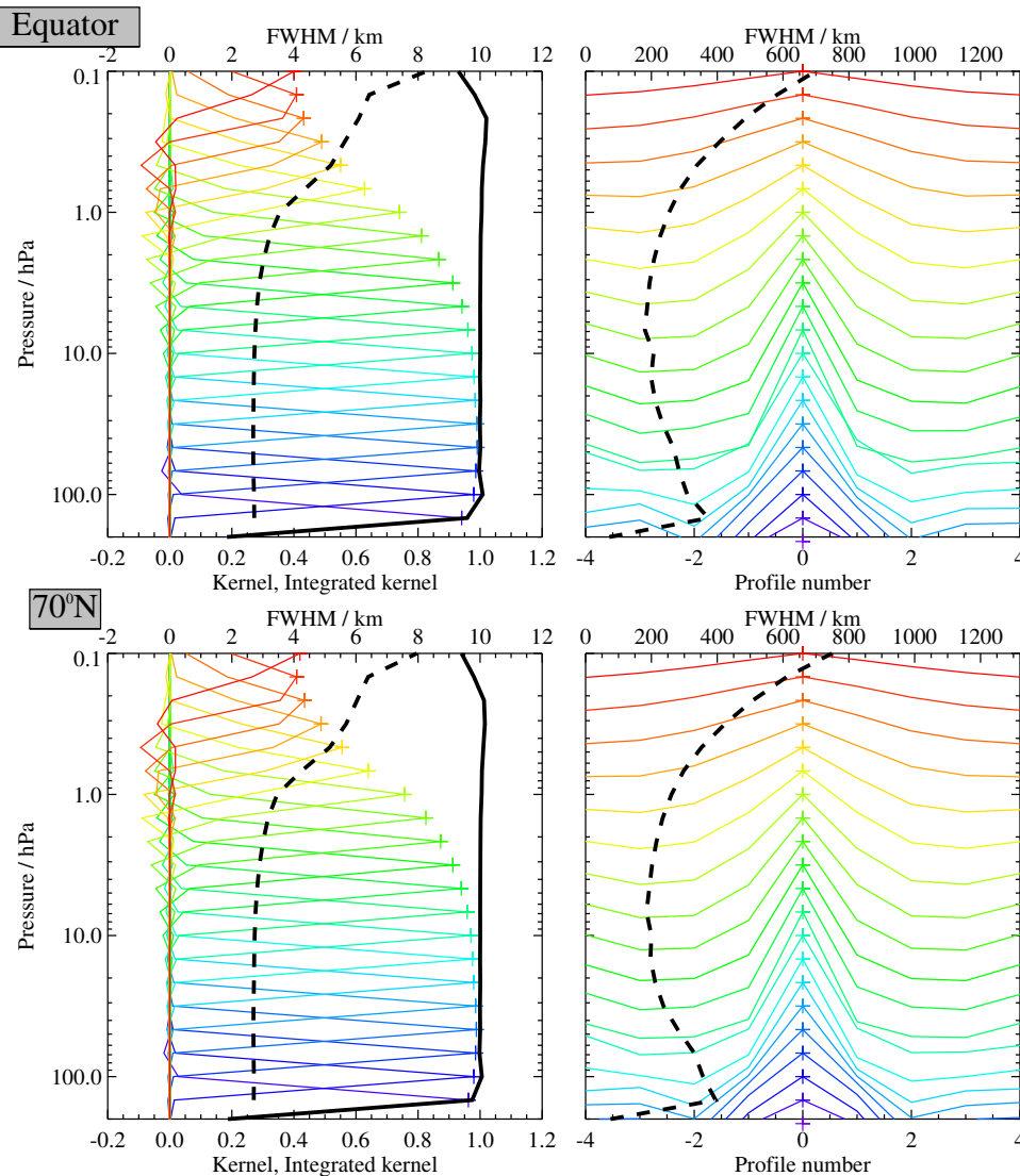
Figure 3.10.3: Typical two-dimensional (vertical and horizontal along-track) averaging kernels for the MLS v5.0x HCl data at the equator (upper) and at 70°N (lower); variation in the averaging kernels is sufficiently small that these are representative of typical profiles. Colored lines show the averaging kernels as a function of MLS retrieval level, indicating the region of the atmosphere from which information is contributing to the measurements on the individual retrieval surfaces, which are denoted by plus signs in corresponding colors. The dashed black line indicates the resolution, determined from the full width at half maximum (FWHM) of the averaging kernels, approximately scaled into kilometers (top axes). (Left) Vertical averaging kernels (integrated in the horizontal dimension for five along-track profiles) and resolution. The solid black line shows the integrated area under each kernel (horizontally and vertically); values near unity imply that the majority of information for that MLS data point has come from the measurements, whereas lower values imply substantial contributions from a priori information. (Right) Horizontal averaging kernels (integrated in the vertical dimension) and resolution. The horizontal averaging kernels are shown scaled such that a unit averaging kernel amplitude is equivalent to a factor of 10 change in pressure.
