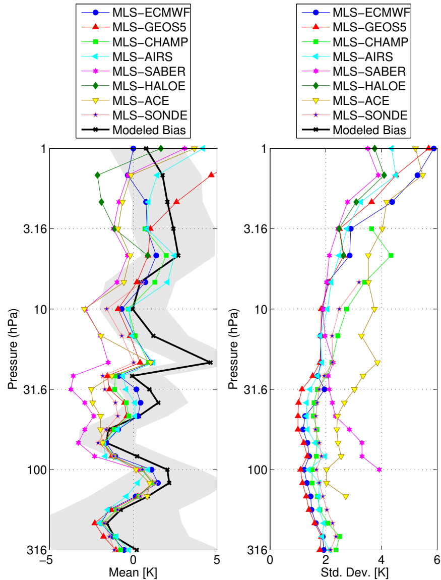
Figure 3.22.5: The left panel shows globally-averaged mean differences between MLS v4.2x temperature and eight correlative data sets. Criteria for coincidences are described in detail in Schwartz et al. [2008]. The right panel shows the global standard deviations about the means.
