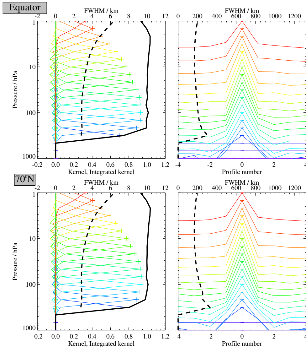
Figure 3.21.2: Typical two-dimensional (vertical and horizontal along-track) averaging kernels for the MLS v5.0x SO 2 data at the equator (upper) and at 70°N (lower); variation in the averaging kernels is sufficiently small that these are representative of typical profiles. Colored lines show the averaging kernels as a function of MLS retrieval level, indicating the region of the atmosphere from which information is contributing to the measurements on the individual retrieval surfaces, which are denoted by plus signs in corresponding colors. The dashed black line indicates the resolution, determined from the full width at half maximum (FWHM) of the averaging kernels, approximately scaled into kilometers (top axes). (Left) Vertical averaging kernels (integrated in the horizontal dimension for five along-track profiles) and resolution. The solid black line shows the integrated area under each kernel (horizontally and vertically); values near unity imply that the majority of information for that MLS data point has come from the measurements, whereas lower values imply substantial contributions from a priori information. (Right) Horizontal averaging kernels (integrated in the vertical dimension) and resolution. The horizontal averaging kernels are shown scaled such that a unit averaging kernel amplitude is equivalent to a factor of 10 change in pressure.
