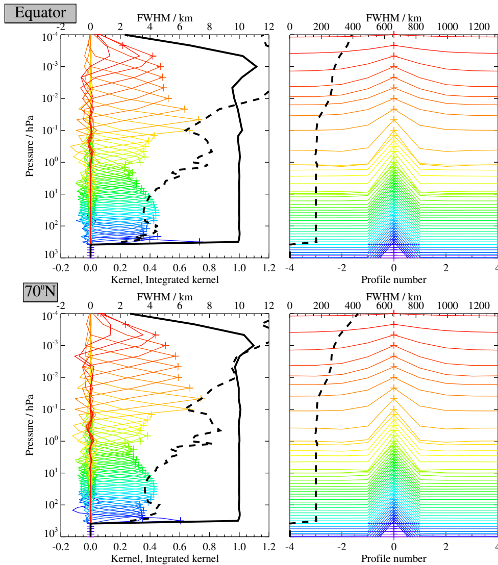
Figure 3.22.4: Typical two-dimensional (vertical and horizontal along-track) averaging kernels for the MLS v5.0x Temperature data at the equator (upper) and at 70°N (lower); variation in the averaging kernels is sufficiently small that these are representative of typical profiles. Colored lines show the averaging kernels as a function of MLS retrieval level, indicating the region of the atmosphere from which information is contributing to the measurements on the individual retrieval surfaces, which are denoted by plus signs in corresponding colors. The dashed black line indicates the resolution, determined from the full width at half maximum (FWHM) of the averaging kernels, approximately scaled into kilometers (top axes). (Left) Vertical averaging kernels (integrated in the horizontal dimension for five along-track profiles) and resolution. The solid black line shows the integrated area under each kernel (horizontally and vertically); values near unity imply that the majority of information for that MLS data point has come from the measurements, whereas lower values imply substantial contributions from a priori information. (Right) Horizontal averaging kernels (integrated in the vertical dimension) and resolution. The horizontal averaging kernels are shown scaled such that a unit averaging kernel amplitude is equivalent to a factor of 10 change in pressure.
