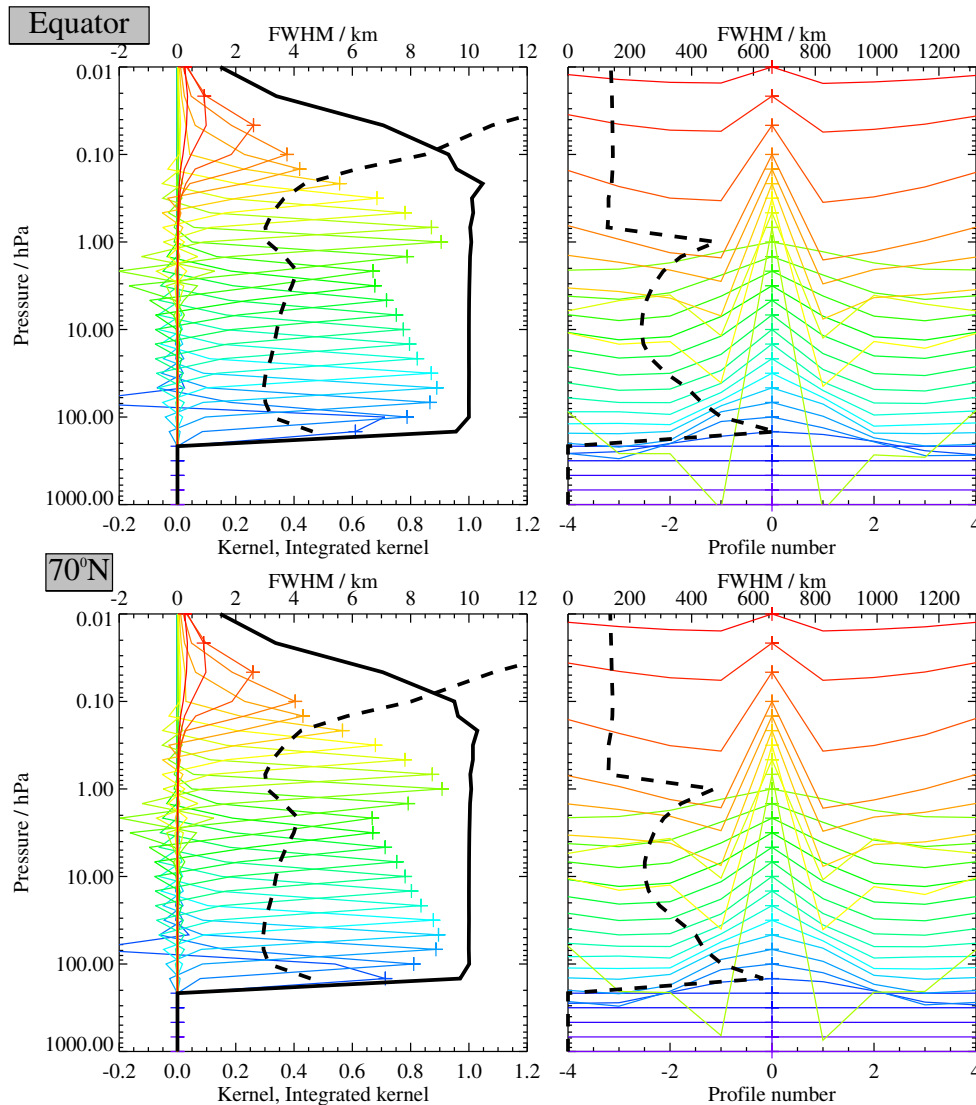
Figure 3.6.1: Typical two-dimensional (vertical and horizontal along-track) averaging kernels for the MLS v5.0x ClO data at the equator (upper) and at 70°N (lower); variation in the averaging kernels is sufficiently small that these are representative of typical profiles. Colored lines show the averaging kernels as a function of MLS retrieval level, indicating the region of the atmosphere from which information is contributing to the measurements on the individual retrieval surfaces, which are denoted by plus signs in corresponding colors. The dashed black line indicates the resolution, determined from the full width at half maximum (FWHM) of the averaging kernels, approximately scaled into kilometers (top axes). (Left) Vertical averaging kernels (integrated in the horizontal dimension for five along-track profiles) and resolution. The solid black line shows the integrated area under each kernel (horizontally and vertically); values near unity imply that the majority of information for that MLS data point has come from the measurements, whereas lower values imply substantial contributions from a priori information. (Right) Horizontal averaging kernels (integrated in the vertical dimension) and resolution. The horizontal averaging kernels are shown scaled such that a unit averaging kernel amplitude is equivalent to a factor of 10 change in pressure.
