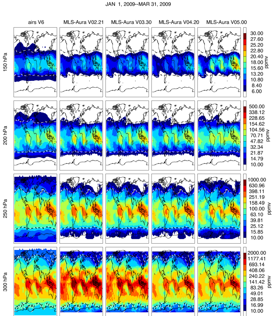
Figure 3.9.7: Mapped fields from AIRS v6 (left), MLS v2.2 (center-left), MLS v3.3 (center), MLS v4.2x (center-right), and MLS v5.0x (right) pressures between 300 and 150 hPa for Jan-Feb-Mar 2009. The black-white lines indicate the tropopause where the region poleward is in the stratosphere. Note that the AIRS measurement is mostly suitable for H 2 O greater than 10 ppmv.
